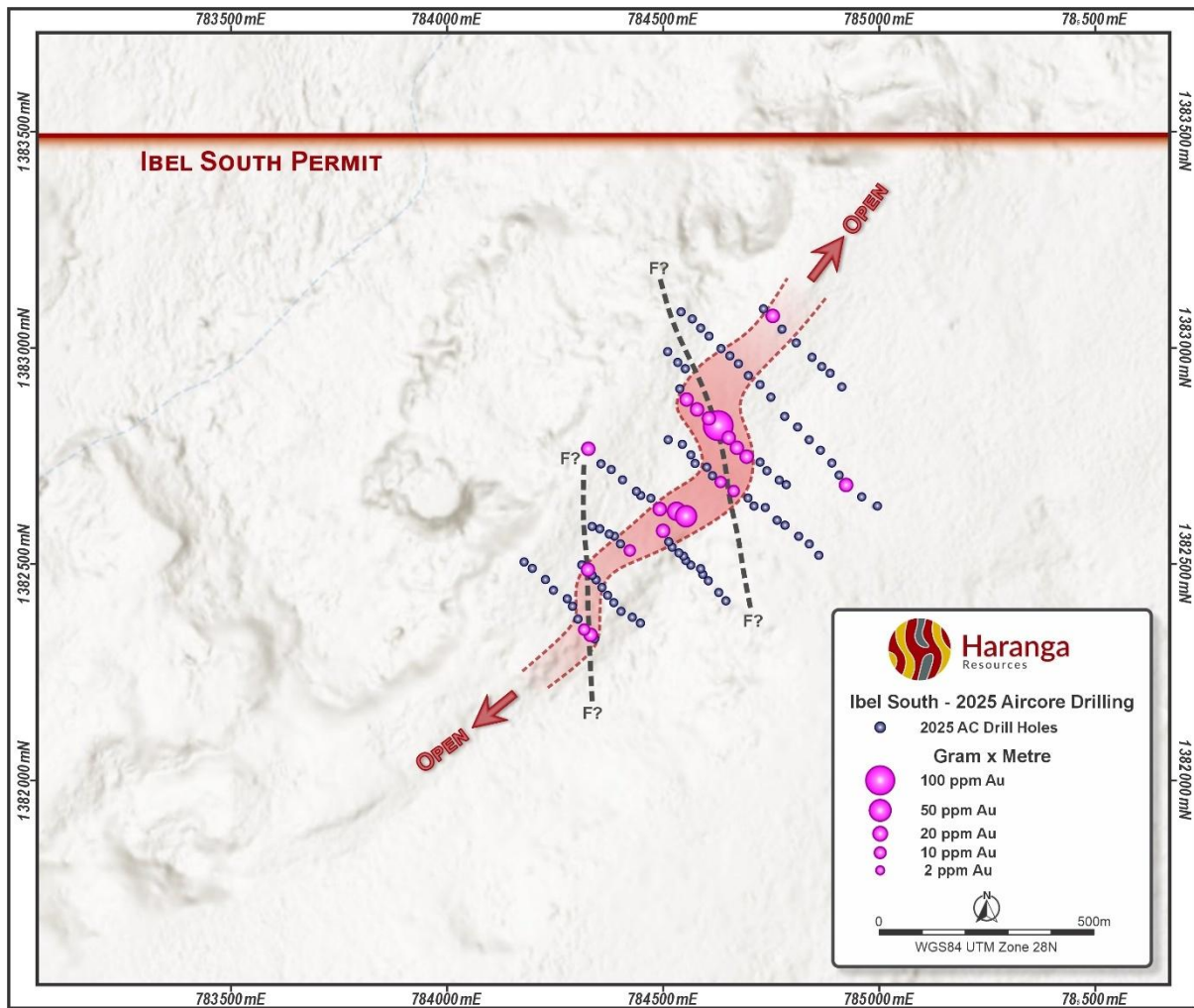
Figure 3: Metal factor ( g \cdot m ) calculated on Phase 1 and 2 AC drilling at Ibel South and possible structural components over TMS Anomaly 3. Dashed lines marked “F?” indicate interpreted locations of potential cross-faulting.
