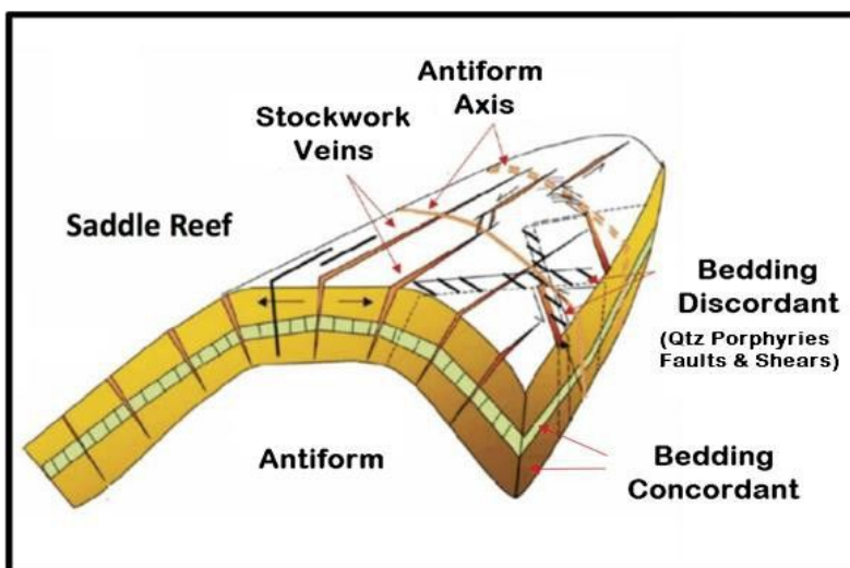
Figure 3 Stock image of antiform saddle reef gold mineralisation, styles at Yidby Gold project.
