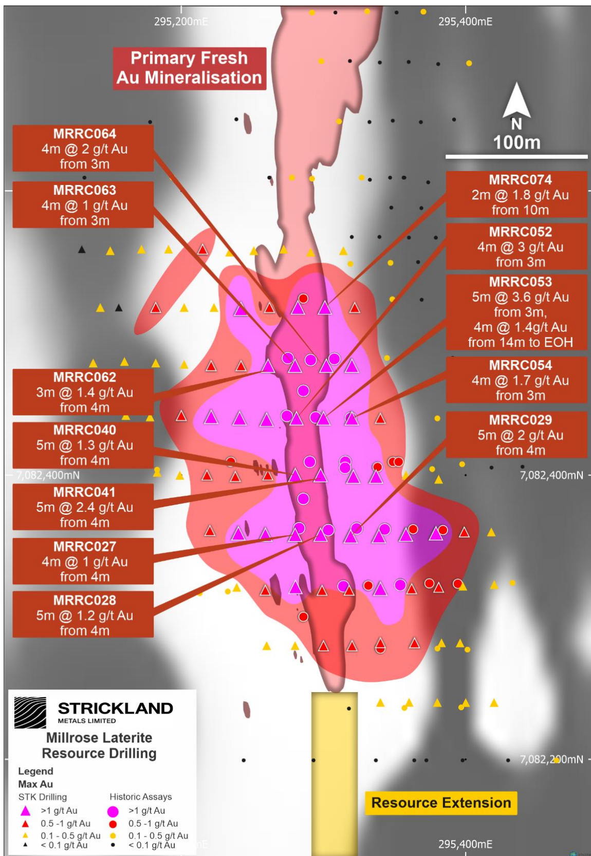
Figure 1: Laterite gold intersections
