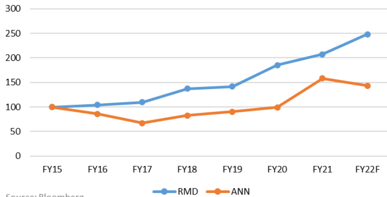
EPS (Indexed)
